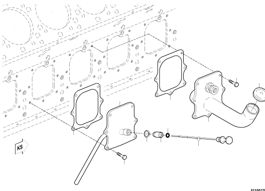
INSPECT PORT COVER FOR OIL DIPSTICK XS527010.00005
